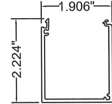
19 Record Hurricane Sensor Cap 6063-T6
