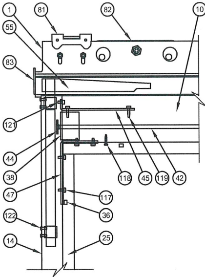
Active Leaf Top Jamb Corner
