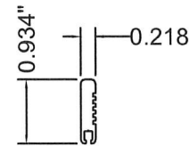
3 Sweep Housing 6063-T5
